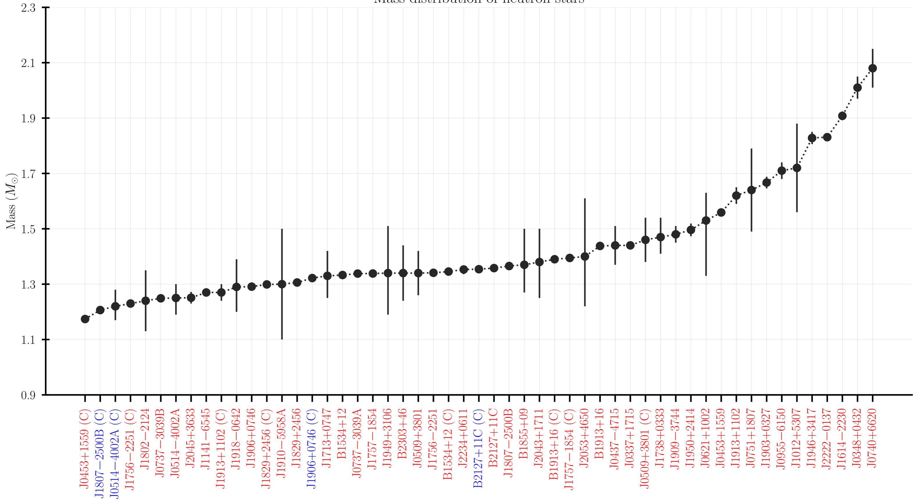
Mass distribution of neutron stars
