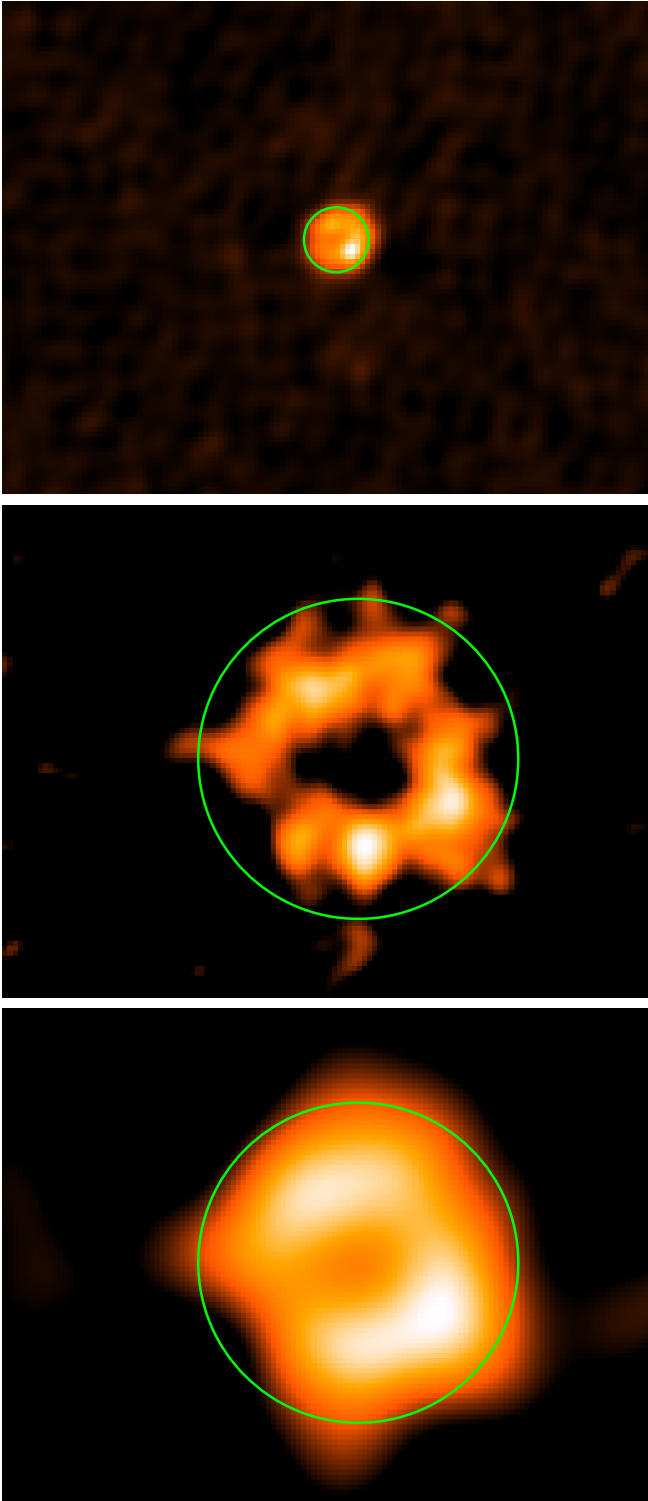
Fig. 4. HSA images at 22 GHz of SN2008iz in May 2008 (top) and April 2009 (middle and bottom). The bottom image is convolved with a dynamic beam of 0.99 mas (i.e. the ratios of beam size and source size are identical in the top and bottom images). The rings denote the best fitted positions and radii from CPM in both epochs, i.e. 320 and 1580 \mu\text{as} .
