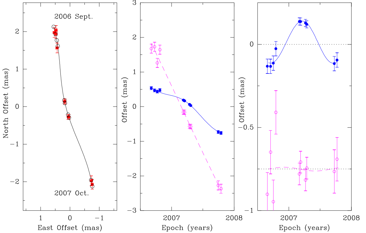
Fig. 2.— Parallax and proper motion data and fits for Sgr B2M. Plotted are position measurements of an \text{H}_2\text{O} maser spot at v_{\text{LSR}} = 66.4 \text{ km s}^{-1} relative to the background source J1745–2820. Left Panel: Positions on the sky ( red circles ) with first and last epochs labeled. The expected positions from the parallax and proper motion fit are indicated ( black circles and solid line ). Middle Panel: East ( filled blue circles and solid line ) and North ( open magenta circles and dashed line ) position offsets and best fit parallax and proper motions fit versus time. The northward data have been offset from the eastward data for clarity. Right Panel: Same as the middle panel , except the best fit proper motion has been removed, allowing the effects of only the parallax to be seen.
