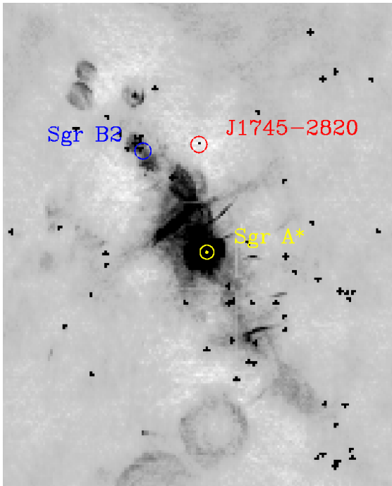
Fig. 1.— VLA 90-cm wavelength image, adapted from LaRosa et al. (2000), with the locations of Sgr A*, Sgr B2, and J1745–2820 indicated. The separation between Sgr B2 and J1745–2820 is \approx 20' .
