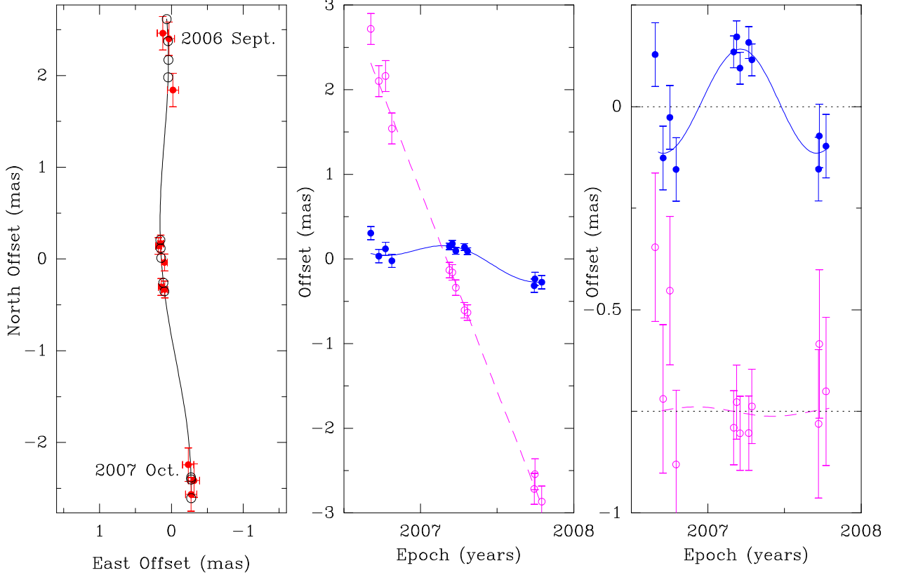
Fig. 3.— Parallax and proper motion data and fits for Sgr B2N. Plotted are position measurements of an H 2 O maser spot at v_{\text{LSR}} = 56.7 \text{ km s}^{-1} relative to the background source J1745–2820. Left Panel: Positions on the sky ( red circles ) with first and last epochs labeled. The expected positions from the parallax and proper motion fit are indicated ( black circles and solid line ). The first epoch point appears to be an outlier and was not used for the fitting. Middle Panel: East ( filled blue circles and solid line ) and North ( open magenta circles and dashed line ) position offsets and best fit parallax and proper motions fit versus time. The northward data have been offset from the eastward data for clarity. Right Panel: Same as the middle panel , except the best fit proper motion has been removed, allowing the effects of only the parallax to be seen.
