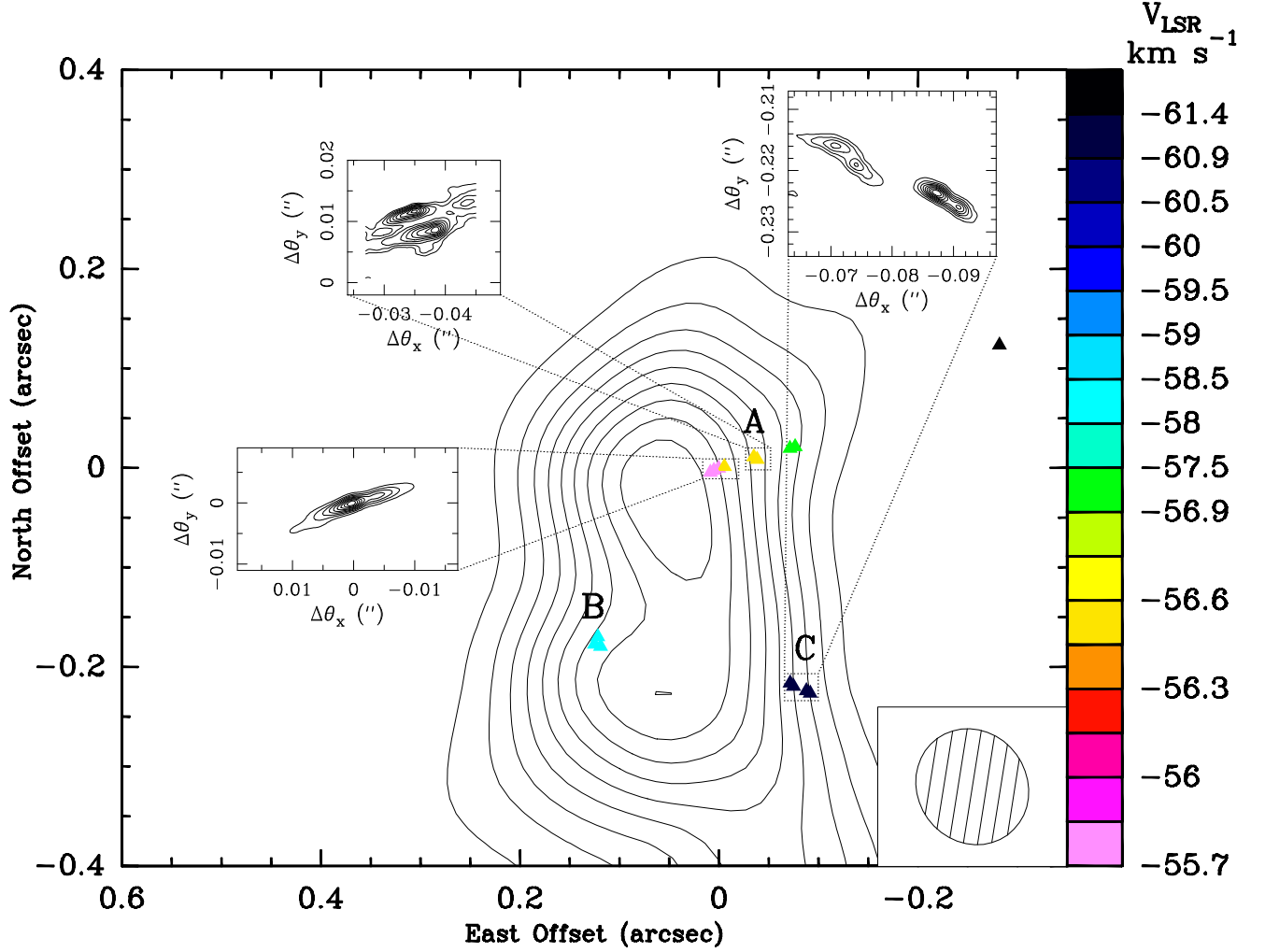
Fig. 8.— NGC 7538 12 GHz methanol maser distribution ( filled triangles ) plotted on a 15 GHz continuum VLA A-configuration image ( contours ) of NGC 7538 IRS1. Plotted levels of the continuum emission are at multiples of 10% of the peak brightness of 23 \text{ mJy beam}^{-1} . Positions are relative to the most intense 12 GHz maser spot, labeled number 1 in Table 4. Different colors are used to indicate the maser LSR velocities, according to the color scale on the right-hand side of the plot. The 6.7 and 12 GHz maser clumps previously detected by Minier et al. (2000, Fig. 1) are labeled with capital letters A, B and C. The insert on the bottom right corner shows the FWHM beam size of the VLA image. Small Panels: The three small panels around the continuum image show the velocity-averaged emission of different groups of intense maser spots at the first observing epoch (2005 Sep. 9). Plotted levels are at multiples of 10% of the (velocity-averaged) spot peak intensity, corresponding to 1.6 \text{ Jy beam}^{-1} , 0.13 \text{ Jy beam}^{-1} and 0.2 \text{ Jy beam}^{-1} for spots shown in the lower left, upper left and upper right panel, respectively.
