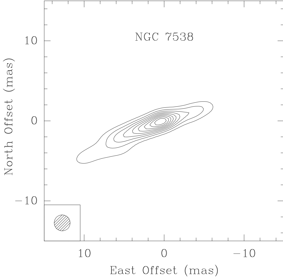
Fig. 1.— Self-calibrated image of the reference maser channel at V_{\text{LSR}} = -55.8 \text{ km s}^{-1} of NGC 7538 for the first epoch (2005 Sep. 9). Contour levels are at multiples of 10% of the peak brightness of 6.2 \text{ Jy beam}^{-1} . The insert in the lower left shows the restoring beam.
