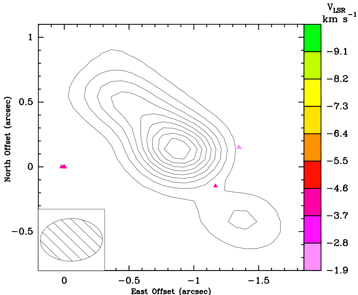
Fig. 7.— Cep A methanol 12 GHz maser distribution ( filled triangles ) plotted on an 8.4 GHz continuum VLA A-configuration image ( contours ) of the Cep A HW2 jet. Plotted levels of the continuum emission are at multiples of 10% of the peak brightness of 5 \text{ mJy beam}^{-1} . Positions are relative to the most intense 12 GHz maser spot (label number 1 in Table 5). Different colors are used to indicate the maser LSR velocities, according to the color scale on the right-hand side of the plot. The color scale was chosen with the source rest velocity set to green and the maximum maser velocity set to purple. The insert at the bottom left corner shows the FWHM beam size of the VLA image. Maser spots in this source are weak and their velocity-averaged emission maps show little structure.
