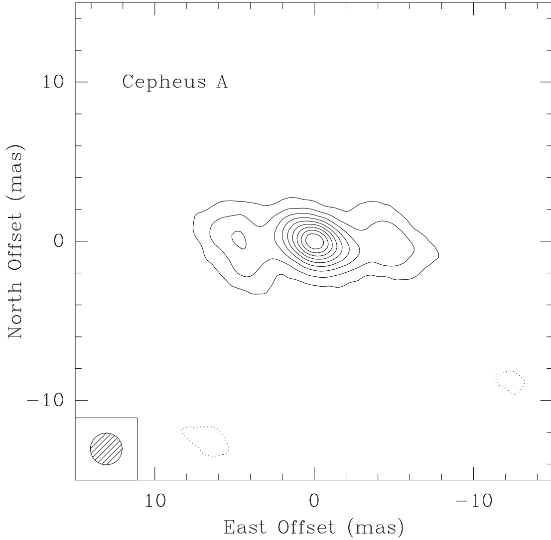
Fig. 4.— Image of the reference maser channel at V_{\text{LSR}} = -4.2 \text{ km s}^{-1} of Cep A for the first epoch (2005 Sep. 9). Contour levels are at multiples of 10% of the peak brightness of 0.9 \text{ Jy beam}^{-1} . The insert in the lower left shows the restoring beam.
