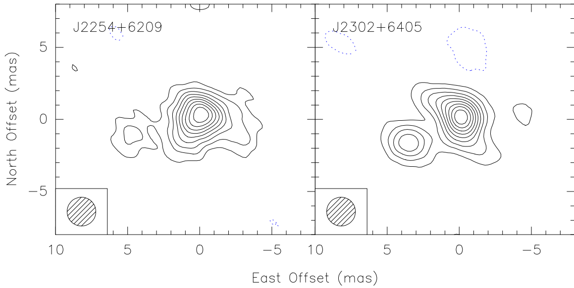
Fig. 5.— Images of the two background continuum sources phase referenced to the Cep A maser. Source names are in the upper left corner and restoring beams are in the lower left corner of each panel. Both images are from the first epoch observations on 2005 Sep. 9. Contour levels of both images are at multiples of 10% of the peak brightness of 0.03 \text{ Jy beam}^{-1} and 0.04 \text{ Jy beam}^{-1} for the J2254+6209 and the J2302+6405 image, respectively.
