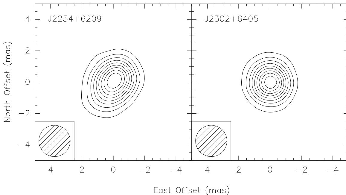
Fig. 2.— Images of the two background continuum sources phase referenced to the NGC 7538 maser. Source names are in the upper left corner and restoring beams are in the lower left corner of each panel. Both images are from the first epoch observations on 2005 Sep. 9. Contour levels of both images are at multiples of 10% of the peak brightness of 0.07 \text{ Jy beam}^{-1} and 0.12 \text{ Jy beam}^{-1} for the J2254+6209 and the J2302+6405 image, respectively.
