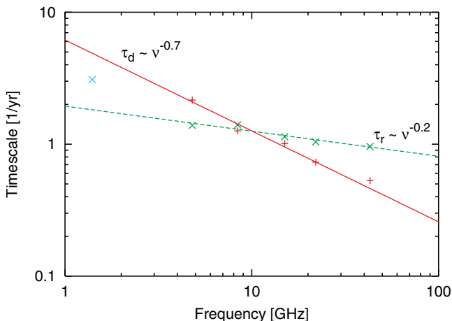
Fig. 8. Rise (×) and decay (+) timescales for all frequencies.
