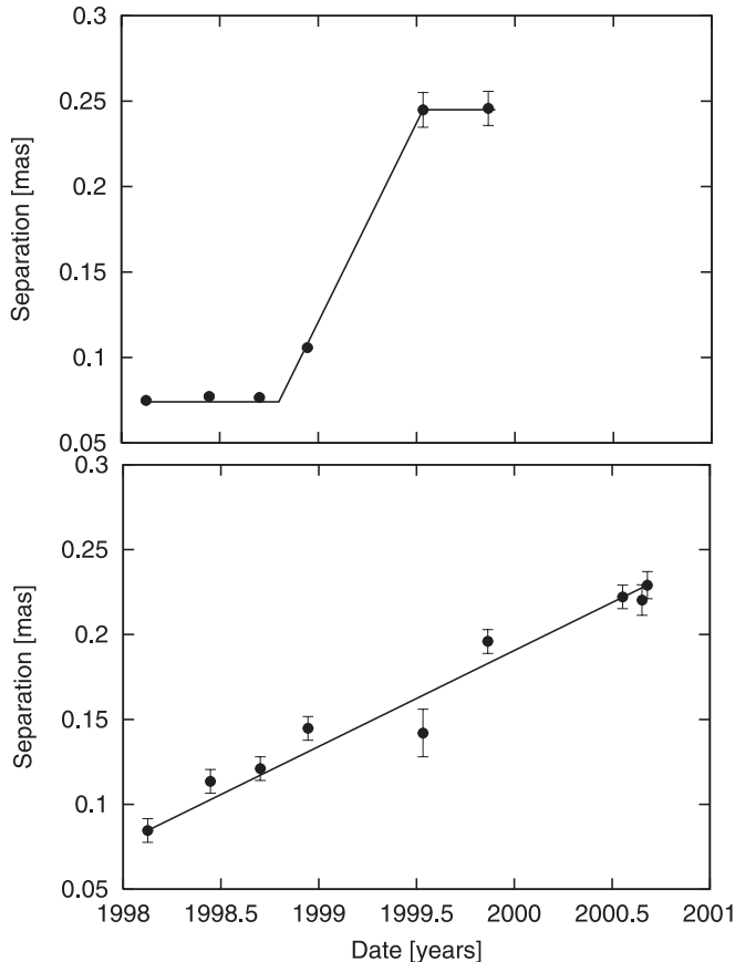
Fig. 13. Component separation at 43 ( upper ) and 15 ( lower ) GHz. The apparent expansion speed is 0.6 c at 15 GHz and 1.25 c at 43 GHz.
