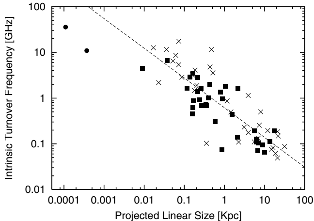
Fig. 14. Intrinsic turnover frequency vs. linear size for GPS and CSS sources. The quasars are represented by crosses, and the galaxies by solid squares. Adapted from O’Dea & Baum (1997). The two circles mark values for III Zw 2 before and after the expansion at 43 GHz.
