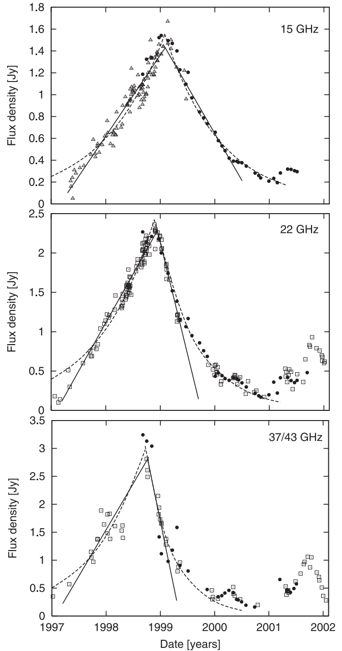
Fig. 6. Radio light curves of the recent flare in III Zw 2 at 15, 22 and 37/43 GHz. Circles are our VLA observations, and triangles are from the Michigan monitoring program, and squares are from the Metsähovi monitoring program. Solid lines are our linear rise and decline fits, while dashed lines are the fitted exponential rise and decay.
