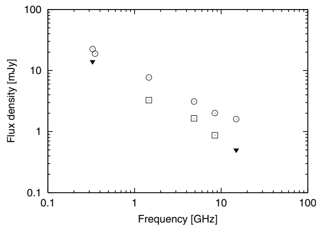
Fig. 3. Spectra of the southwestern (circles) and northeastern (squares) radio lobes. The black triangles are upper limits for the northeastern lobe.
