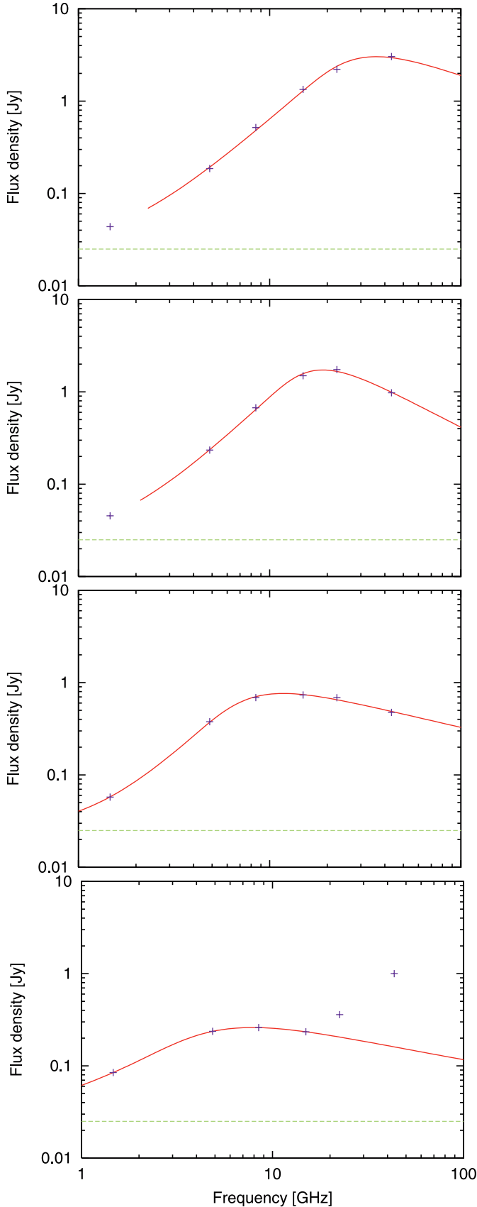
Fig. 9. Spectra of III Zw 2 on 4 November 1998 ( top ), 22 February 1999 ( middle ), 12 November 1999 ( middle ), and 30 January 2001 ( bottom ) together with the quiescent spectrum (horizontal line) and the best fit spectrum.
