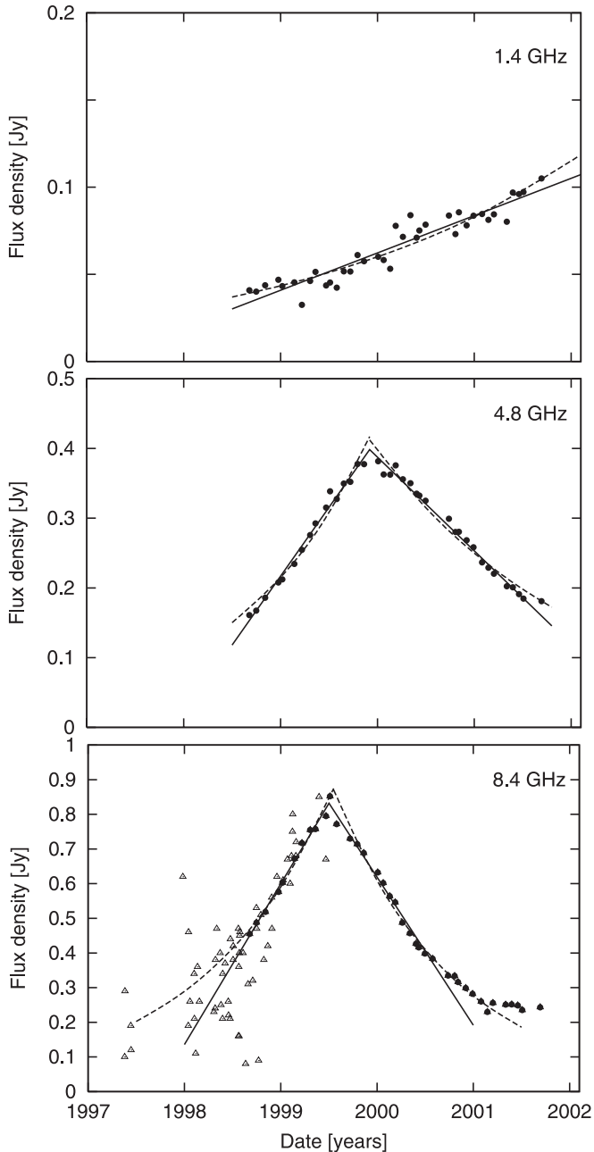
Fig. 5. Radio light curves of the recent flare in III Zw 2 at 1.4, 4.8 and 8.4 GHz. Circles are our VLA observations, and triangles are from the Michigan monitoring program. Solid lines are our linear rise and decline fits, while dashed lines are the fitted exponential rise and decay.
