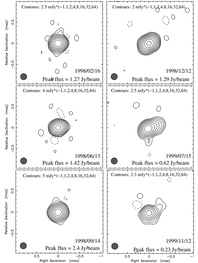
Fig. 12. All six VLBA maps of III Zw 2 at 43 GHz convolved with a superresolved circular beam of 150 \mu\text{as} .
