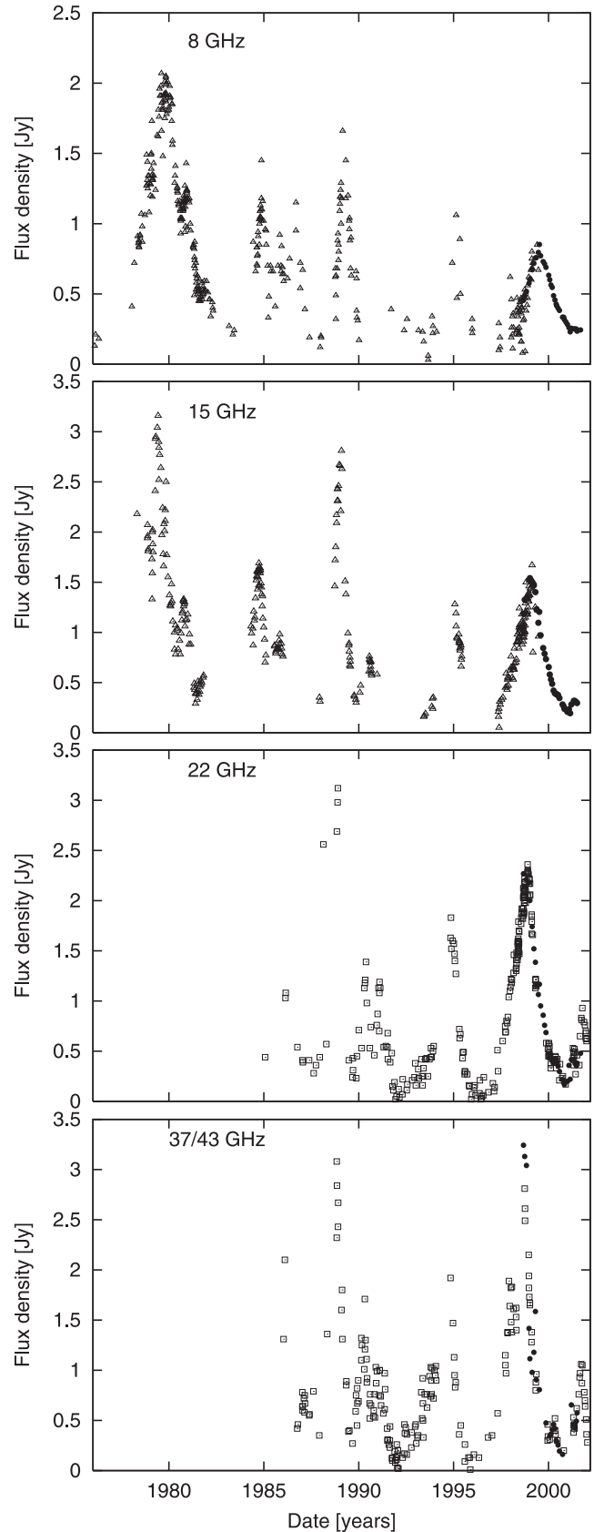
Fig. 4. Radio light curves of III Zw 2. The triangles at 8 and 15 GHz are from the Michigan monitoring program, the squares at 22 and 37 GHz are from the Metsähovi monitoring program. The circles are our VLA observations at 8, 15, 22, and 43 GHz.
