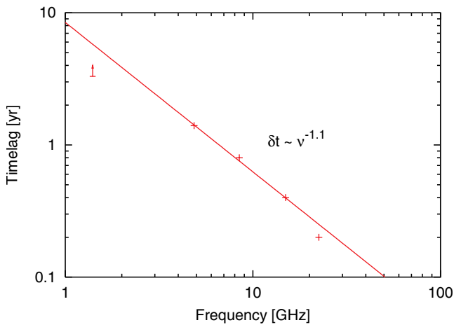
Fig. 7. Time-lag between the peak at 43 GHz and the peak at the other frequencies. The data point at 1.4 GHz is a lower limit.
