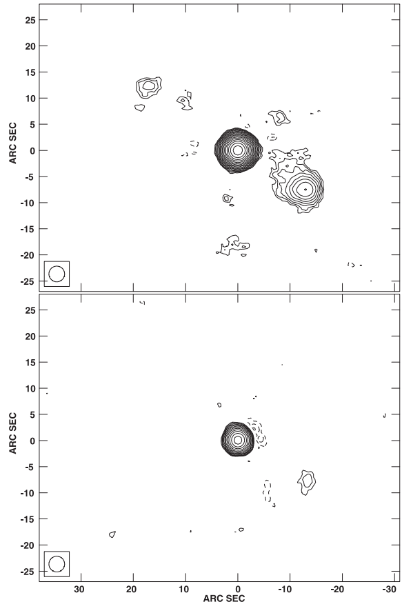
Fig. 2. Combined VLA map of 11 epochs (A, B, C and D-array) of III Zw 2 at 8.4 GHz ( top ) and 15 GHz ( bottom ). All maps were convolved with a beam of 2 \times 2 arcsec to detect faint extended emission. The contours start at 0.12 mJy at 8.4 GHz and 0.6 mJy at 15 GHz, and increase with a factor of \sqrt{2} .
