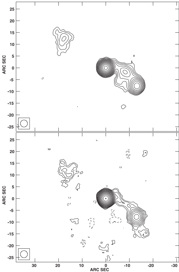
Fig. 1. Combined VLA map of 11 epochs (A, B, C and D-array) of III Zw 2 at 1.4 GHz ( top ) and at 4.8 GHz ( bottom ). All maps were convolved with a beam of 2 \times 2 arcsec to detect faint extended emission. The contours start at 0.26 mJy at 1.4 GHz and 0.15 mJy at 4.8 GHz, and increase with a factor of \sqrt{2} .
