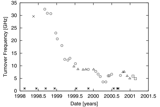
Fig. 10. Evolution of the “turnover frequency” \nu_0 . Circles mark epochs with 6 observed frequencies (1.4–43 GHz) and triangles epochs with 5 observed frequencies (1.4–22 GHz). In the last two epochs only 4 frequencies (1.4–15 GHz) were used because of a new outburst at high frequencies. The cross is the turnover frequency of the spectrum in May 1998, where the 1–43 GHz data is taken from Falcke et al. (1999). The asterisks mark the epochs of our VLBA observations.
