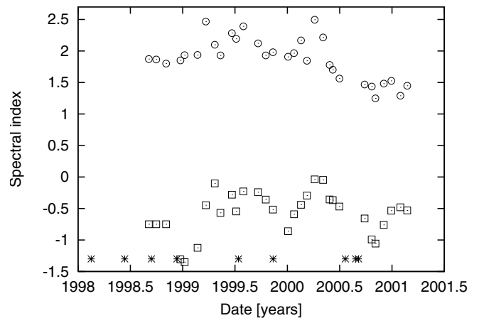
Fig. 11. Evolution of the spectral indices k (circles) and l (squares). The asterisks mark the epochs of our VLBA observations.
