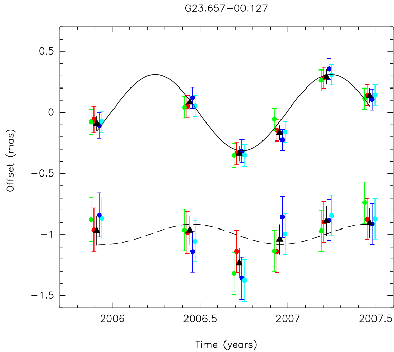
Fig. 3. Position offsets of four spots (filled circles) in right ascension (top) and declination (bottom) after removing the proper motion, superposed on the combined parallax fit model for all maser spots in Table 2. The data points are slightly shifted in time for clarity. Also shown are the average positions of all spots (black triangles).
