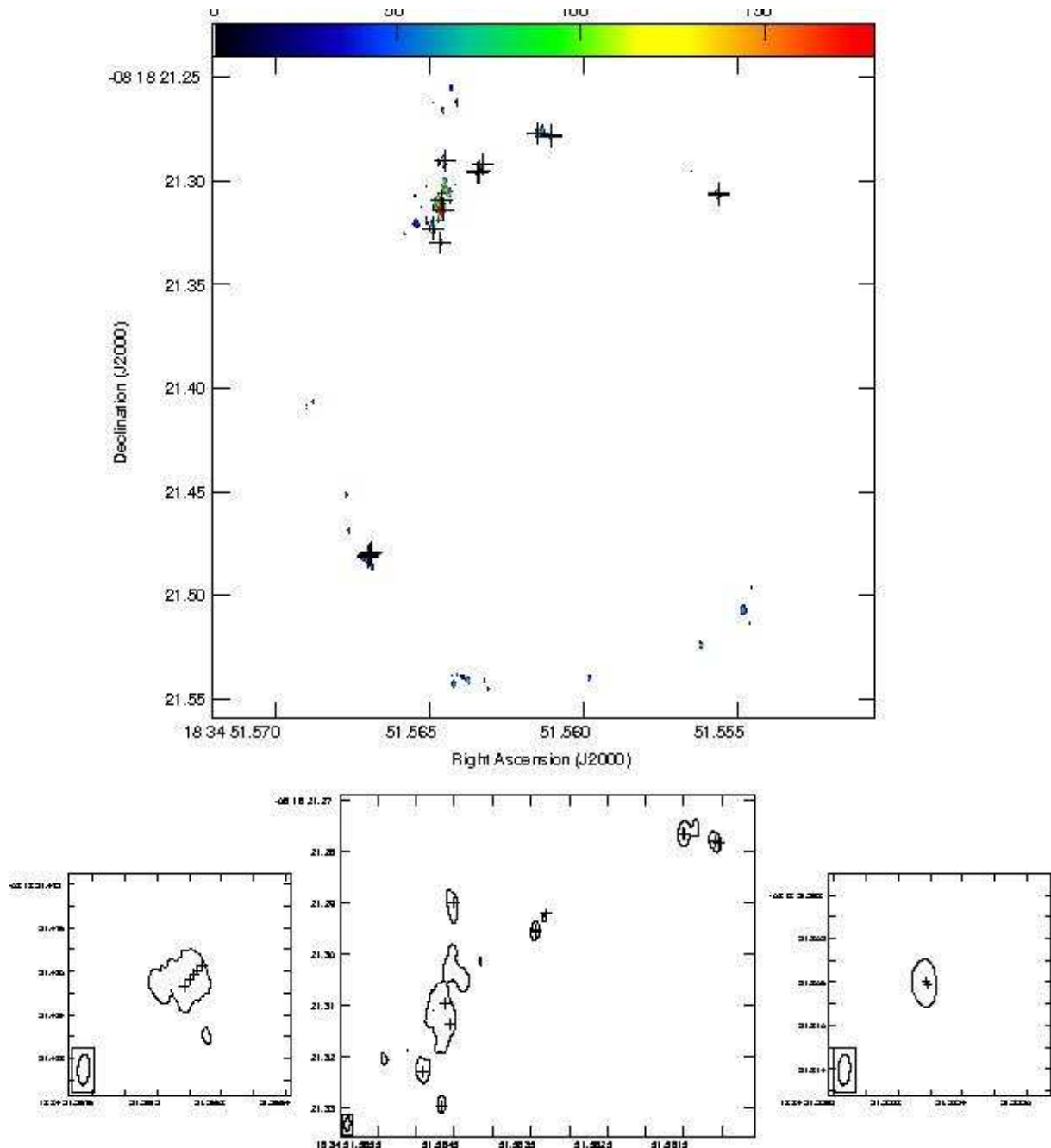
Fig. 1. Top: Total intensity (“zeroth” moment) map of 12.2 GHz methanol maser from G23.657–00.127 from 2007 June 19 using the VLBA. The color scale (in the electronic version) varies linearly from 0 to 180 Jy beam -1 m s -1 . The 19 crosses represent spots that were chosen for the parallax estimation (Table 2). Bottom: The enlarged views of the masering regions. The contours correspond to the value of 10% of the peak (i.e., 38.6 Jy beam -1 m s -1 ). The beam is indicated by the ellipses in the bottom left-hand corners.
