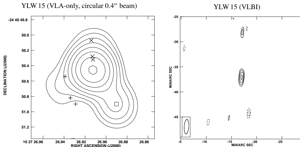
Fig. 1. Left: VLA-only map of YLW 15 (B array data, April 2005), restored with a circular 0.4'' beam. The proper motions of the two components as determined by Curiel et al. (2003) are indicated (years 1990, 2000, and 2002 form north to south for both sources) together with the chosen VLBI correlation position (box). The contour lines delineate multiples of 0.1 \text{ mJy} ( \sim 4\sigma ), increasing by factors of \sqrt{2} . Right: Weak source found in the VLBI data close to the putative position of YLW 15 YLW 2 at RA 16^{\text{h}}27^{\text{m}}26.88875^{\text{s}} DEC -24^{\circ}40'50.937'' . The source reaches a significance of \sim 9\sigma . The contour lines delineate multiples of 3\sigma , increasing by factors of \sqrt{2} . The 1\sigma rms noise level is 15.4 \mu\text{Jy} . Both figures from Forbrich et al. (2007).
