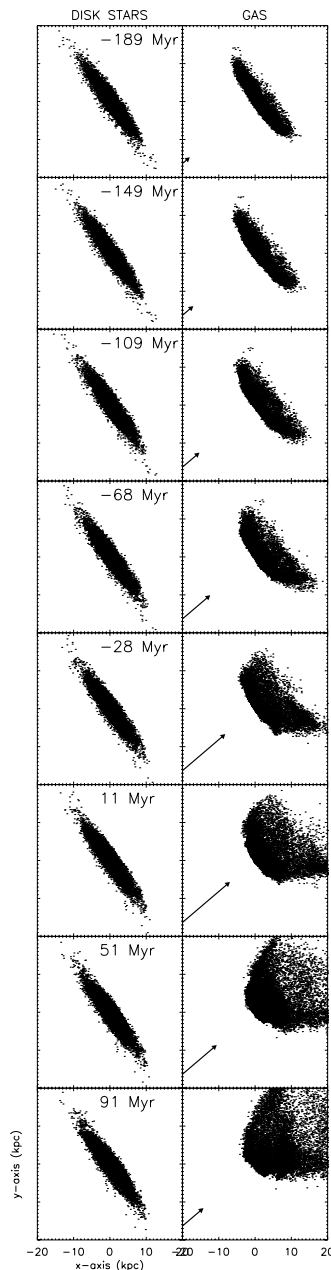
Fig. 5. Evolution of the model stellar (1st column) and gas disk (2nd column). The major axis position angle and inclination of NGC 4522 are \text{PA} = 214^\circ and i = 80^\circ , respectively. The arrow indicates the direction of ram pressure, i.e. it is opposite to the galaxy's velocity vector, and its size is proportional to \rho v_{\text{gal}}^2 . Maximum ram pressure occurs at t = 0 \text{ Myr} . The timestep of each snapshot is marked in each panel showing the stellar disk.
