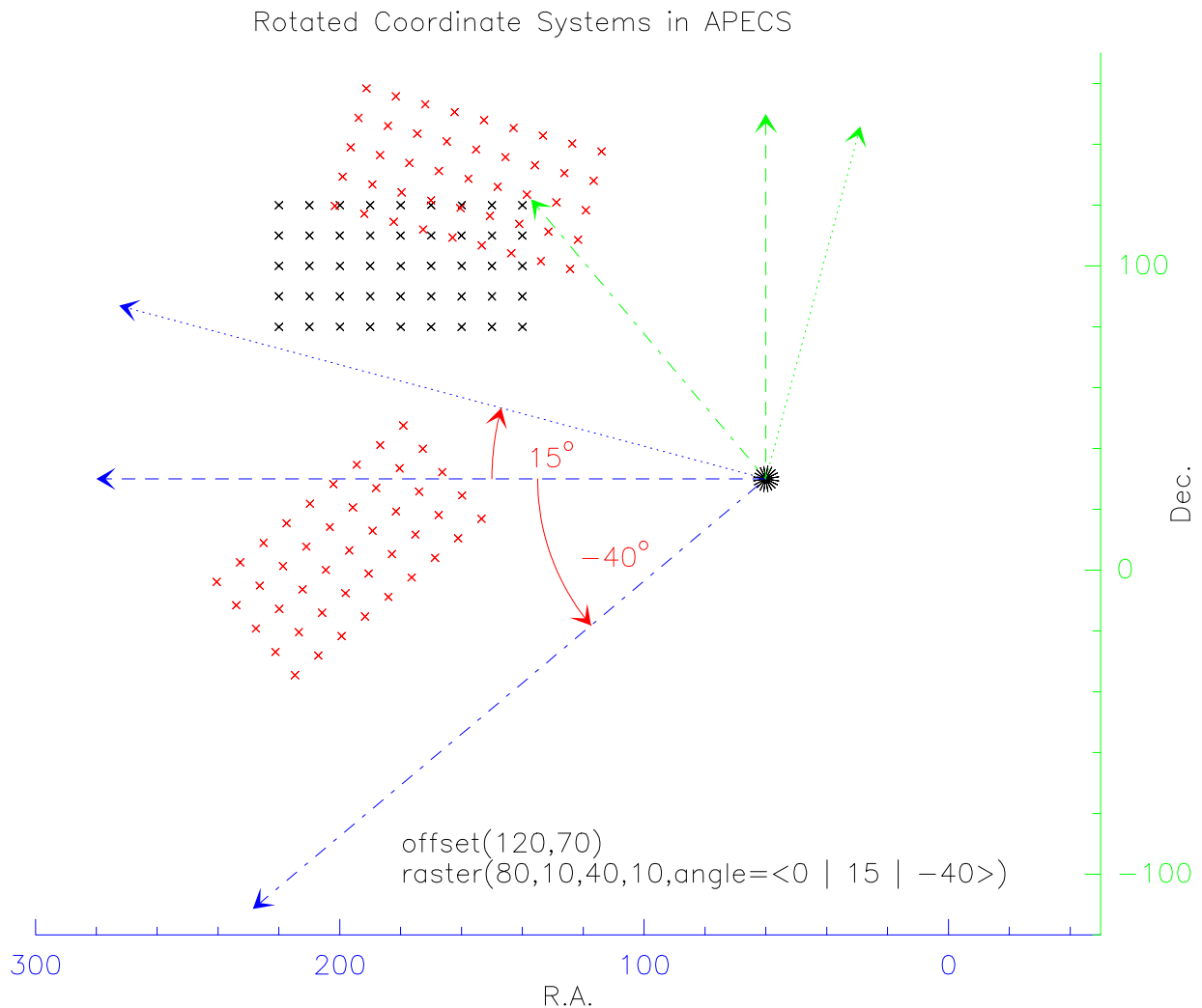
Figure 3.1: Rotated coordinate systems in APECS shown for a raster command. The same angle definition is used for all other patterns.
