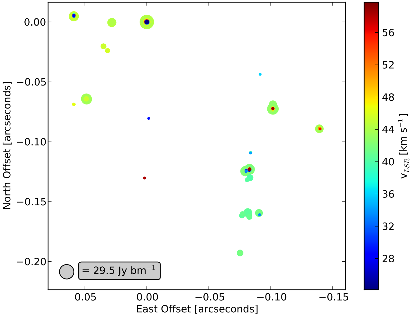
G035.20-1.73 CH 3 OH_6.7GHz on 2012-11-05 (0,0)=19:01:45.54197,+01:13:32.687 (J2000)
