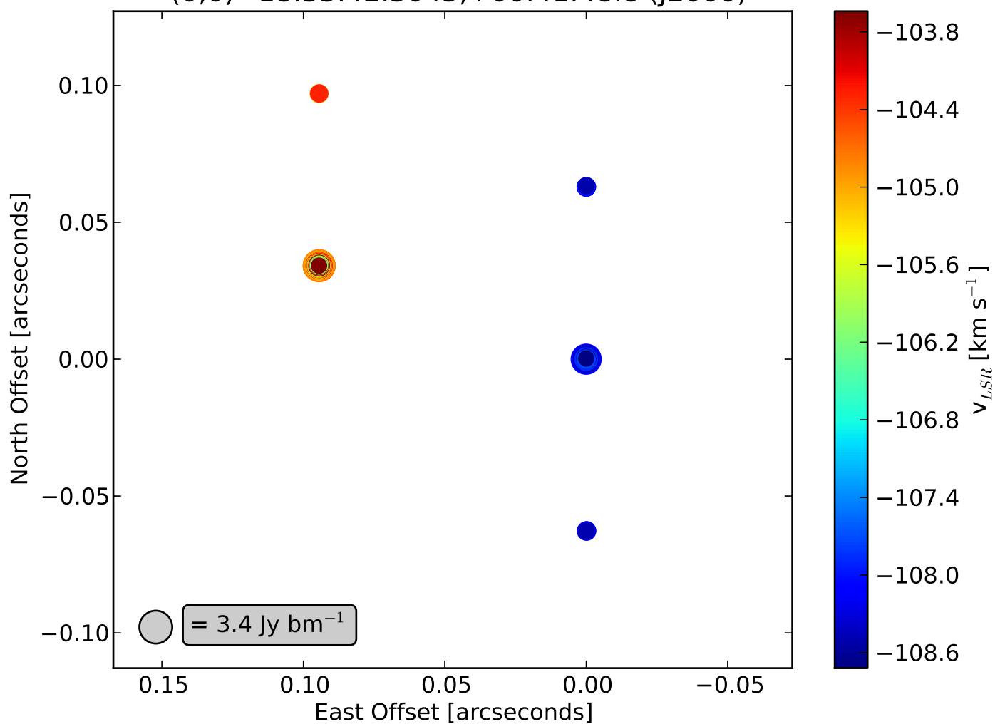
G033.81-0.18 H2O on 2013-11-06 (0,0)=18:53:42.3045,+00:41:48.8 (J2000)
