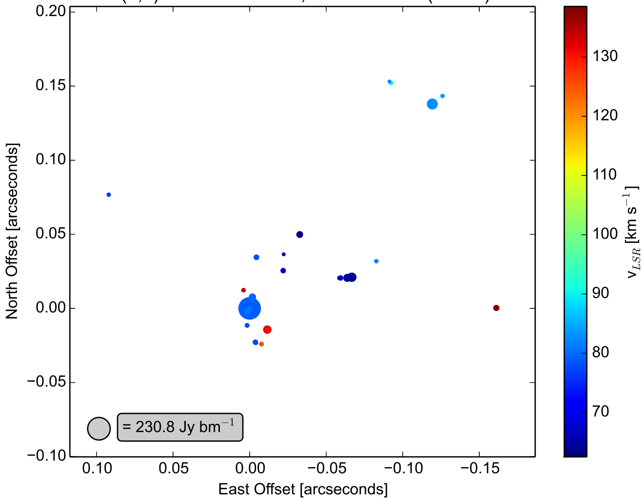
G023.20-0.37 H 2 O on 2014-03-22 (0,0)=18:34:55.17939,-08:49:15.206 (J2000)
