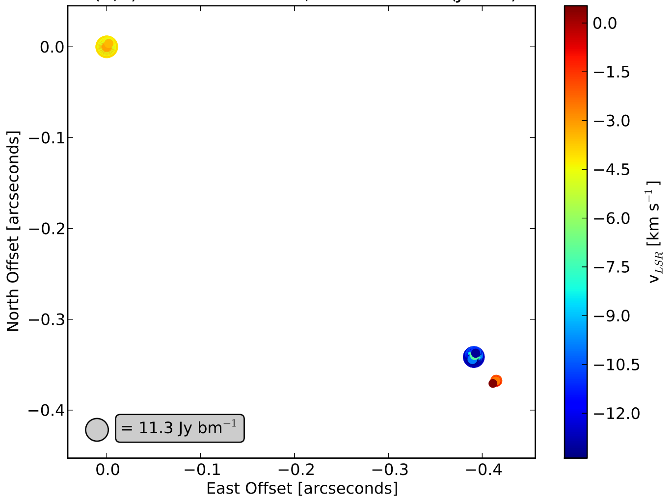
G008.83-0.02 H 2 O on 2014-03-16 (0,0)=18:05:25.70107,-21:19:25.002 (J2000)
