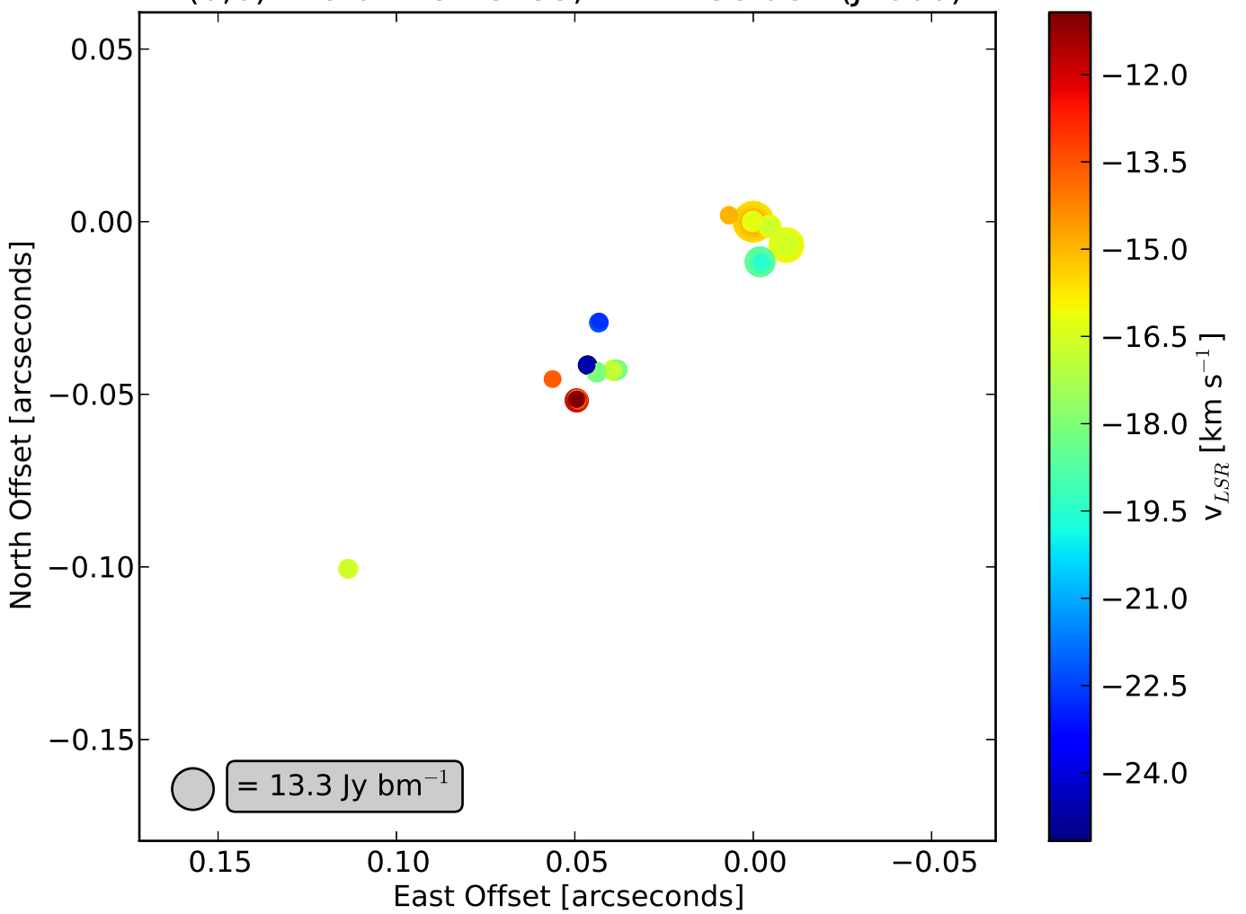
G007.47+0.05 H 2 O on 2014-03-18 (0,0)=18:02:13.18233,-22:27:58.981 (J2000)
