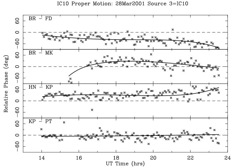
Fig. 1. Observed residual phases (stars) and model phase (line) for the baselines Brewster – Fort Davis, Brewster – Mauna Kea, Hancock – Kitt Peak and Kitt Peak – Pie Town. The model allows for a relative position offset and a single vertical atmospheric delay.
