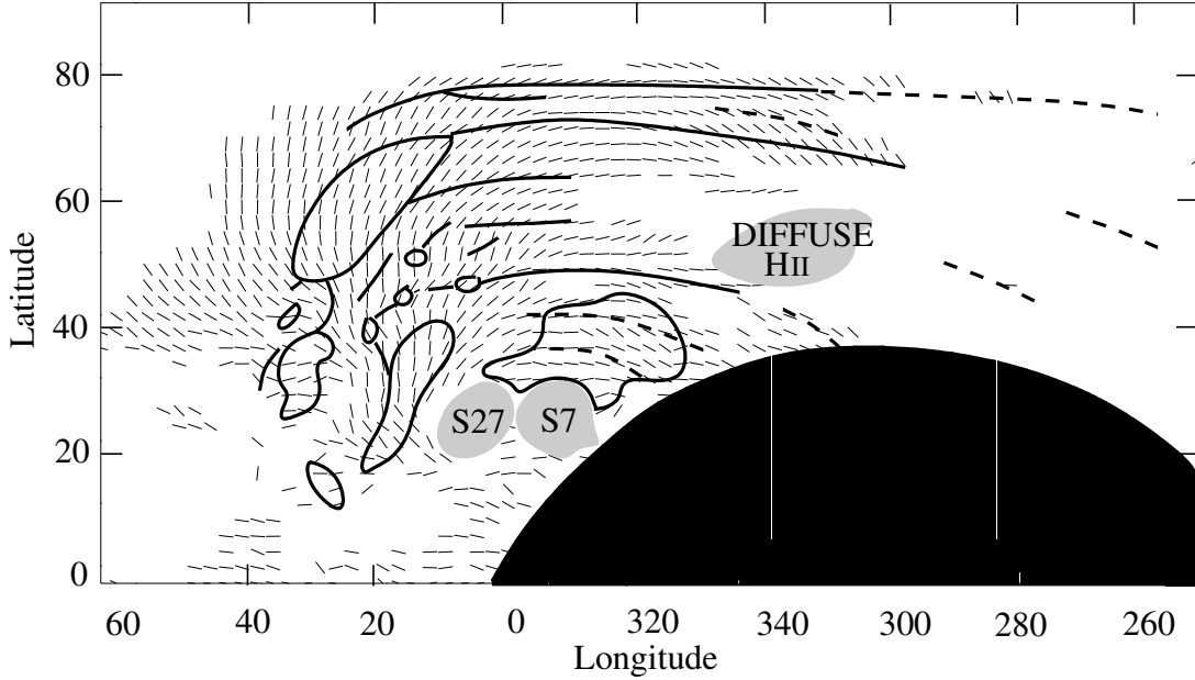
Figure 7.3: Sketch highlighting the filaments of the North-Polar Spur with B-vectors of polarized emission at 1.4 GHz overlayed. The shadowed areas are regions of enhanced H \alpha emission. Vectors of equal length are shown for PI \geq 140 mK. Solid lines mark contours of filaments in the polarized intensity map, whereas dashed lines indicate less confined filaments.
