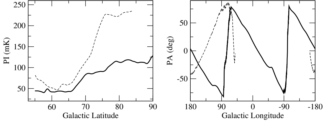
Figure 7.10: The left panel shows the observed increase of polarized intensity toward the northern (thick line) and southern (dashed line) Galactic poles. To avoid confusion the North-Polar Spur was excluded in this plot. The right panel shows the polarization angle (E-vectors) along two Galactic longitude cuts for b \geq 80^\circ (thick line) and b \leq -80^\circ (dashed line).
