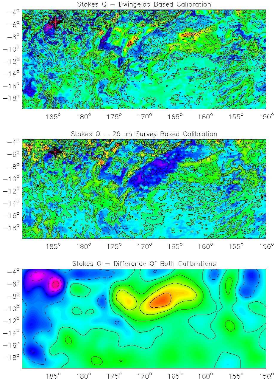
Figure 6.2: Stokes Q : contours run in steps of 100 mK for the two upper images and in steps of 50 mK for the bottom image. Colour cuts are the same for the two upper images. Dashed contours indicate negative Q values.
