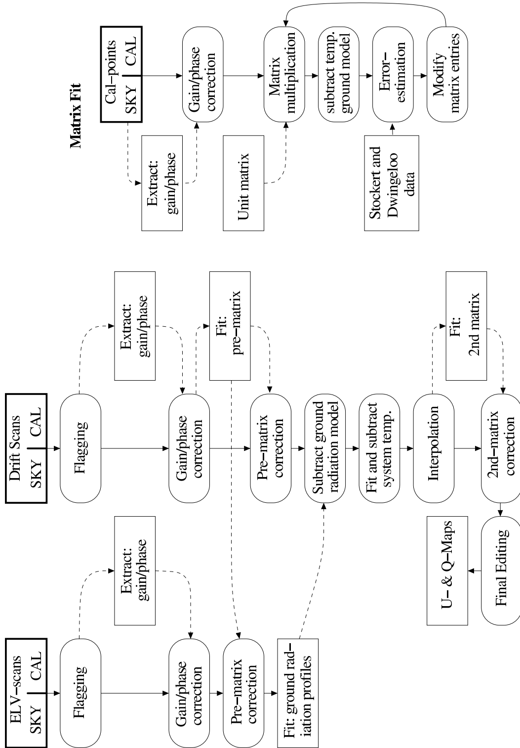
Figure 4.1: Reduction chain
