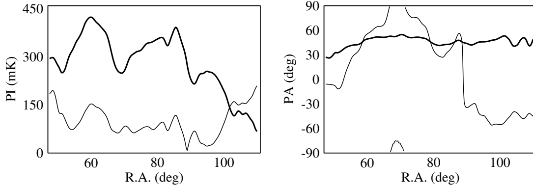
Figure 1.5: The effect of missing large-scale structures: The left panel shows the polarized intensity (PI) taken from a survey drift scan at 57.5^\circ declination with large-scale structures (thick line) and without (thin line). The right panel displays the same for the polarization angle (PA). For this example the large-scale structure is approximated by averaging of Stokes U and Q over the right ascension interval displayed.
